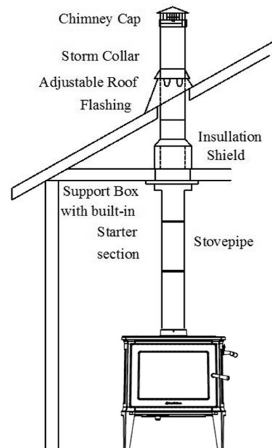
One story house installation with attic.
