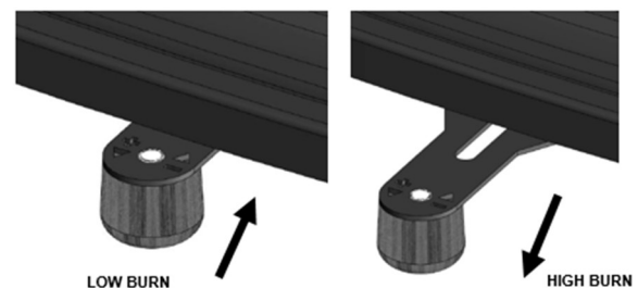
Figure 10 – Air Control
