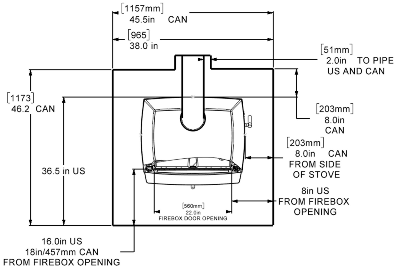
Figure 3 – Hearth Dimensions
