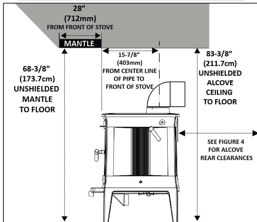
Figure 5: Trim, Mantle, and Alcove Clearances
