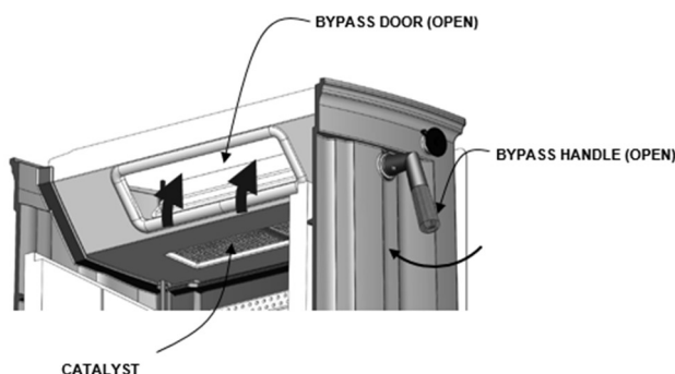
Figure 12 – Bypass Open
