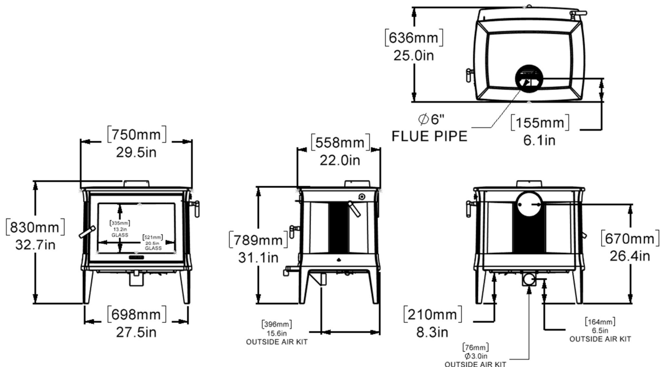
Figure 1 – Green Mountain 80 Dimensions
