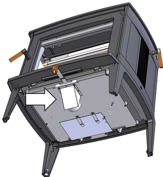
Figure 4 – Outside Air Kit Detail
