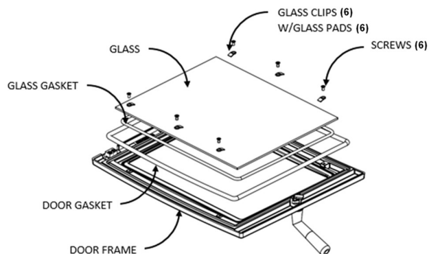
Figure 22: Front Door assembly
