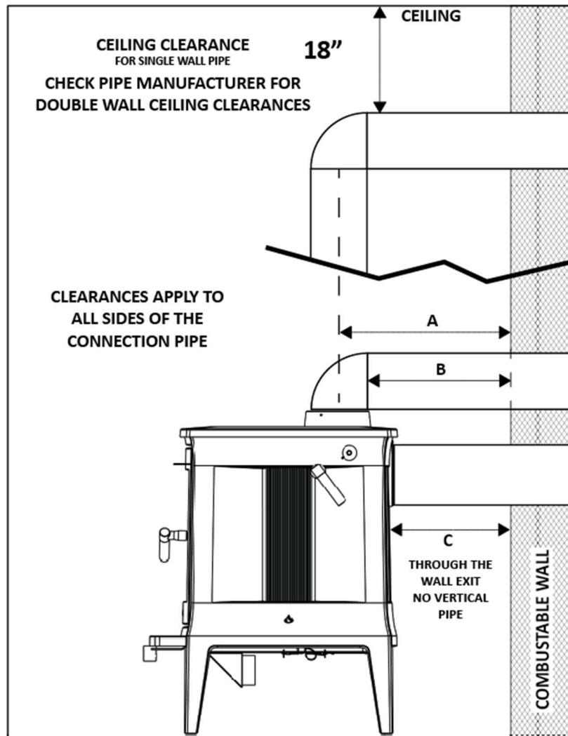
Figure 6 Rear Exit Install Clearances
