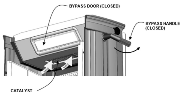
Figure 11 – Bypass Closed
