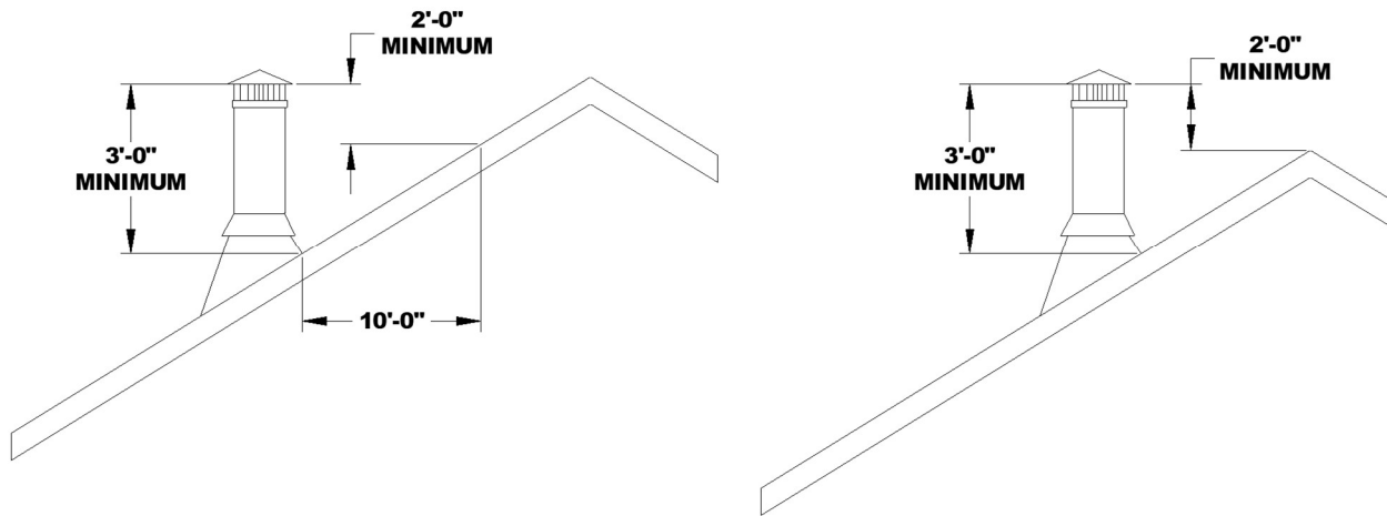
Figure 5 - Chimney Height Requirements
