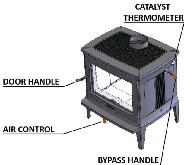
Figure 9 - Controls & Features
