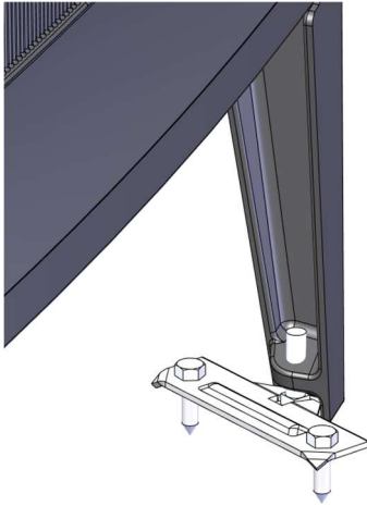
Figure 7 - Lock Down Detail
