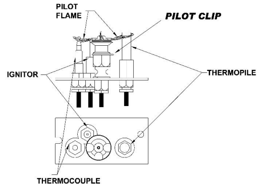
Figure 11: Pilot Assembly Detail
