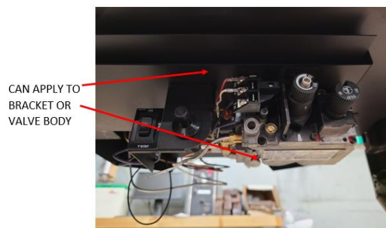
Figure 16 – Valve Warning Label Location
