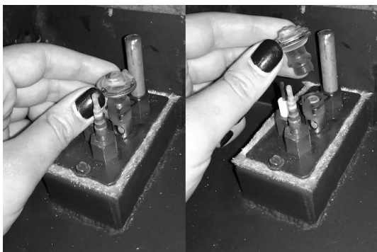
Figure 6 – Removing Pilot Burner Hood
