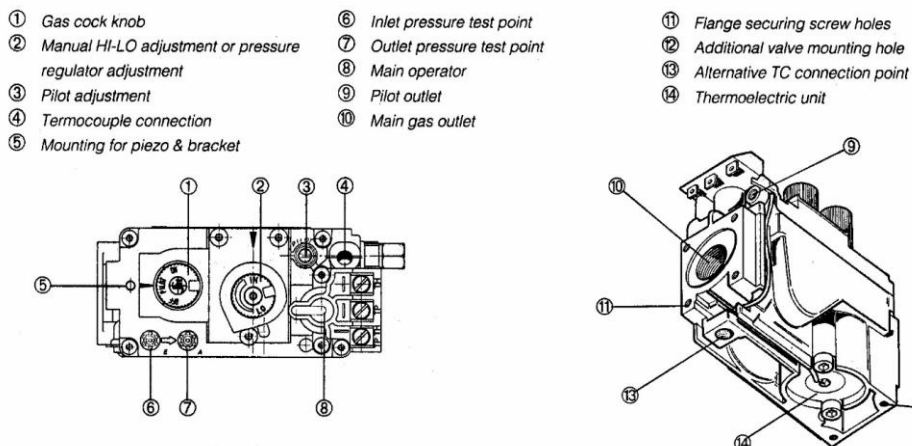
Figure 1 – SIT 820 Valve
