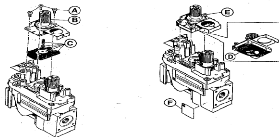
Figure 4 – Valve Conversion Kit
