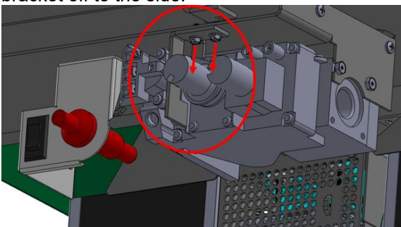
Figure 3 – Stopper Bracket Removal
