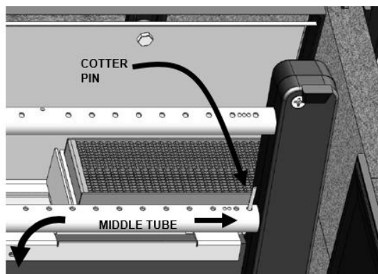
Figure 20 – Removing the Middle Air Tube
