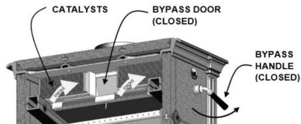
Figure 15 – Bypass Closed
