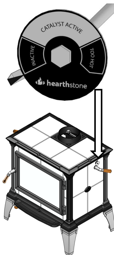
Figure 17 – Catalyst Probe
