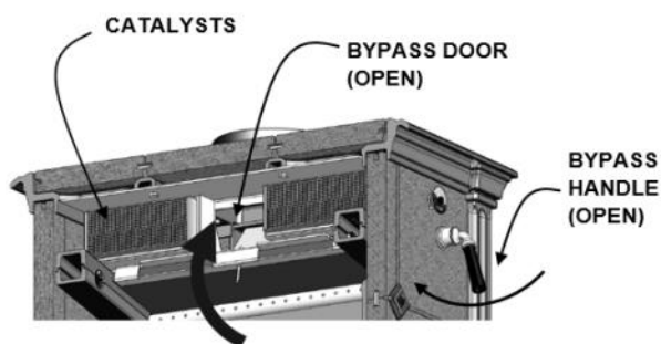
Figure 16 – Bypass Open
