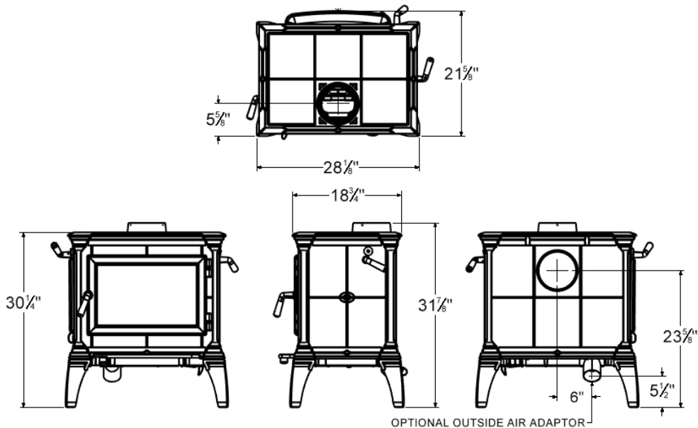
Figure 1 – Heritage 8024 Dimensions
