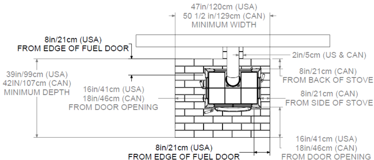
Figure 2 – Hearth Dimensions
