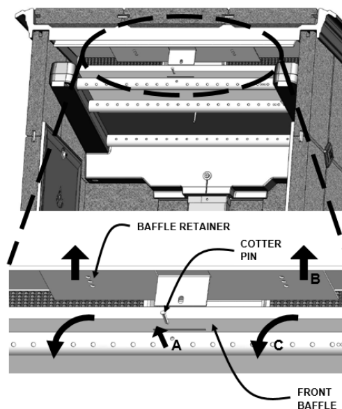
Figure 19 – Removing the Front Baffle
