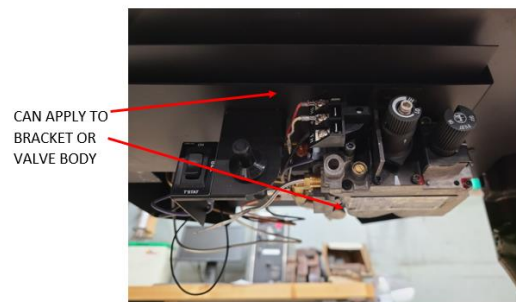
Figure 16 – Valve Warning Label Location
