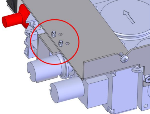
Figure 5 – Stopper Bracket Reinstall Hole Location
