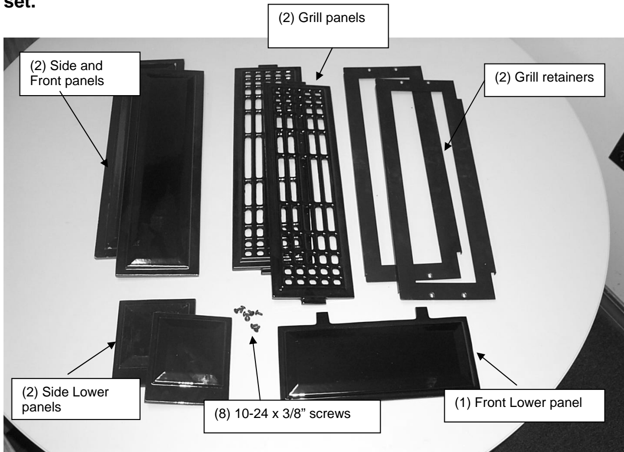
Figure 2 - Keepsake Components
