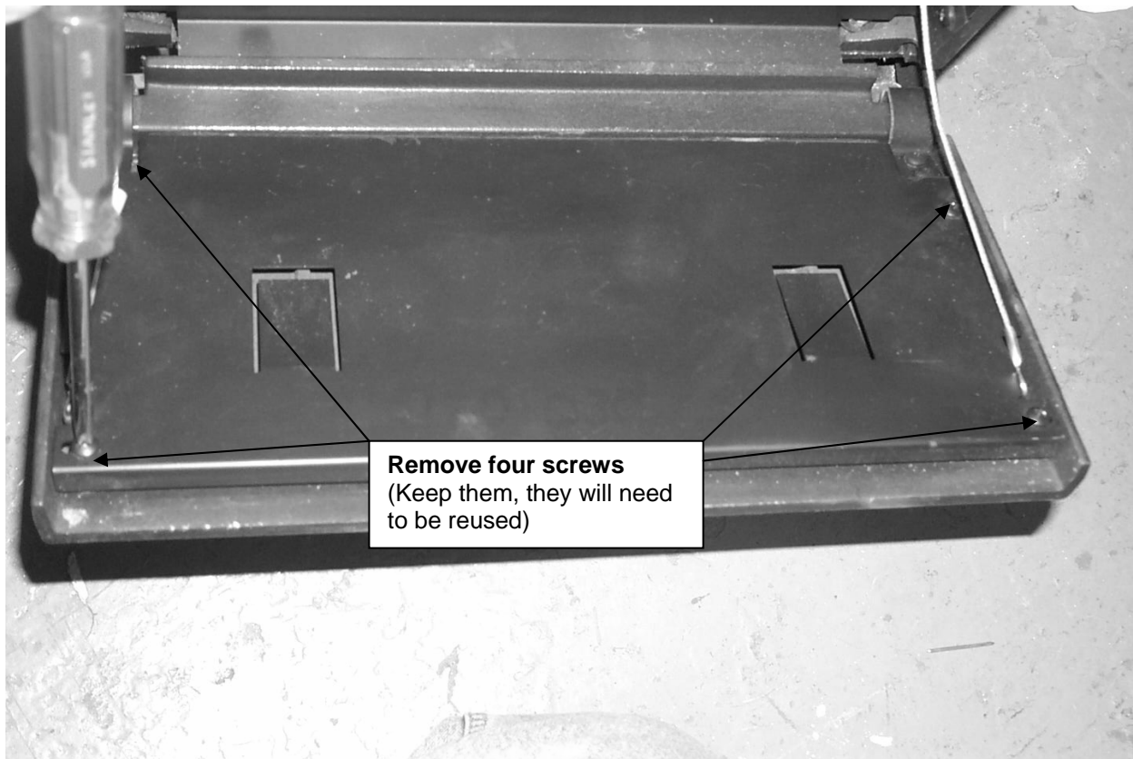
Figure 5 - Front Lower Panel Installation
