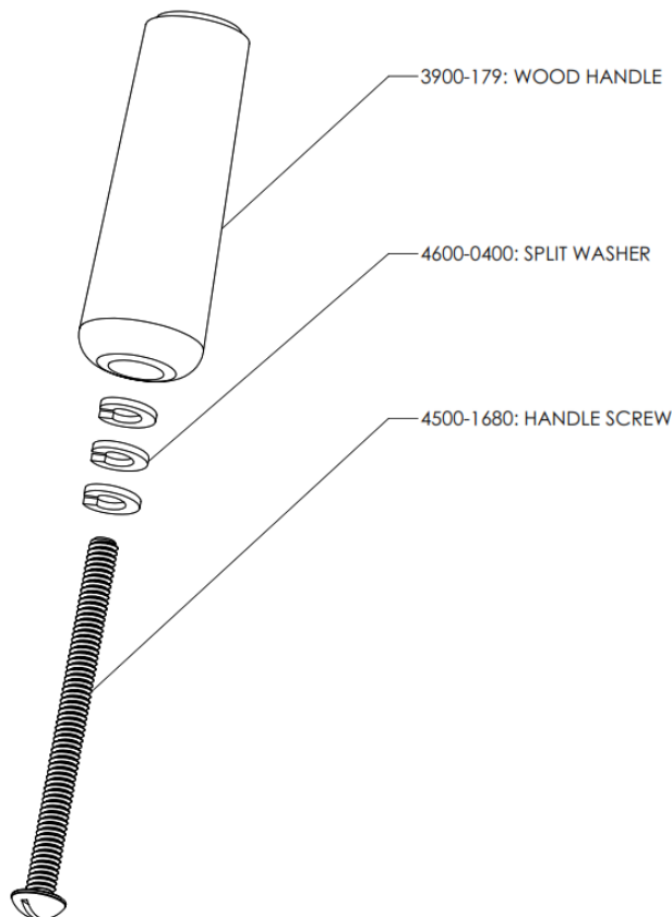
Figure 1: Handle Components
