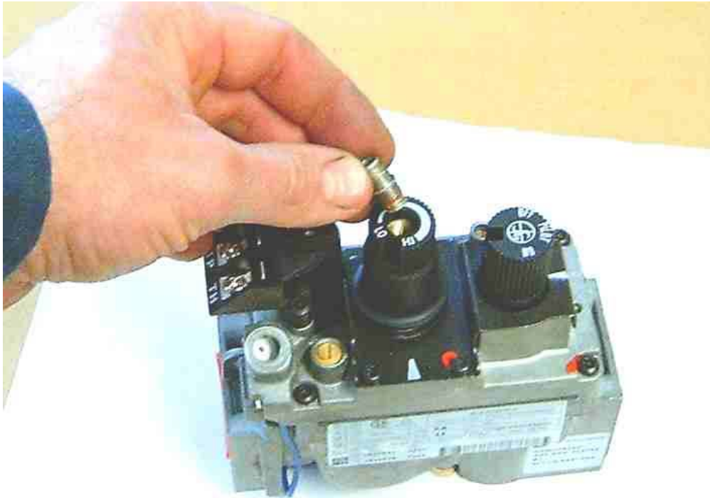
Figure 3 - Rotate the plug 180 degrees and turn it back into the valve. Snug with allen wrench.
