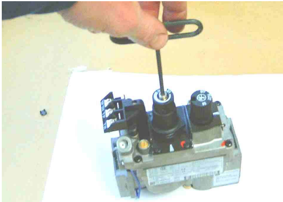
Figure 2 - Loosen and remove the conversion plug with the allen wrench.
