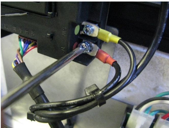
Disconnect the Red TC spade connector.
